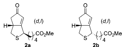
Figure 3. Major ( 2a ) and minor ( 2b ) products of the Pauson–Khand reaction.
