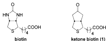
Figure 1. Biotin and ketone biotin.
