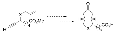
Scheme 3. Possible Use of the Pauson–Khand Reaction to Synthesize Analogues of 1
