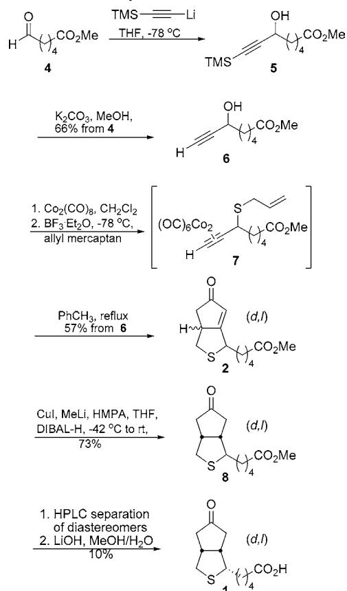
Scheme 2. Synthesis of Ketone Biotin ( 1 )
