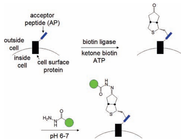
Figure 2. Labeling of cell surface proteins (black rectangle) linked to an acceptor peptide (blue rectangle) with ketone biotin and hydrazide-bearing biophysical probes (green circle). 2
