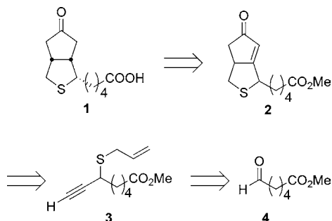
Scheme 1. Retrosynthetic Analysis of 1
